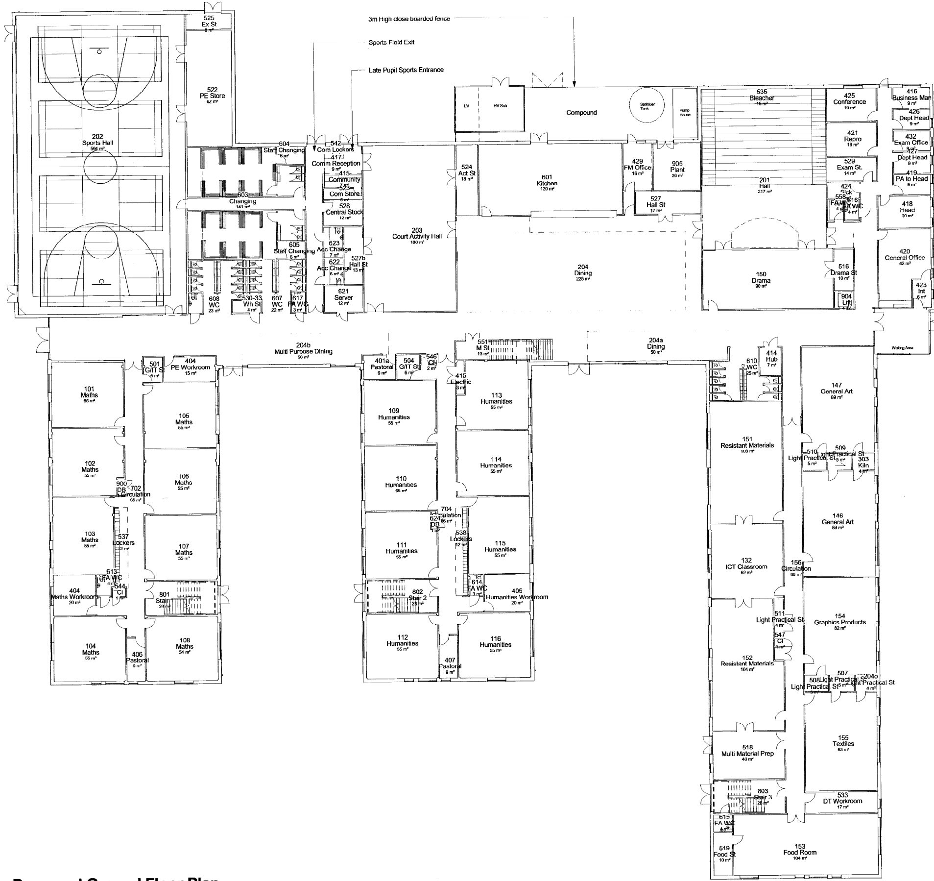
1 Proposed Ground Floor Plan 1 : 200
